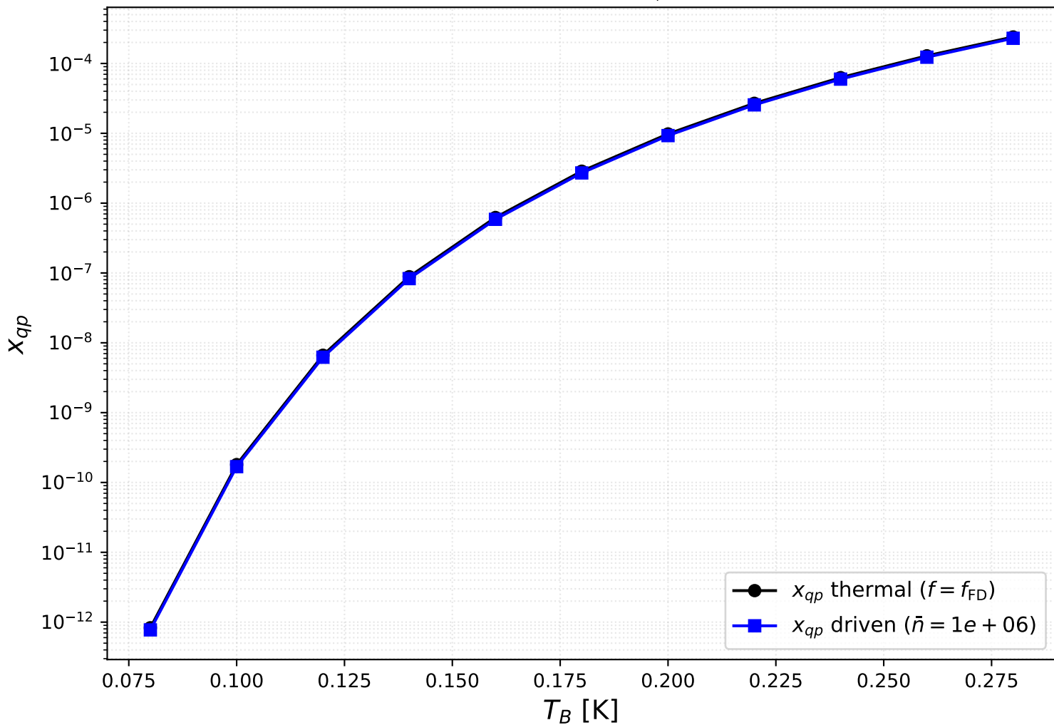
Fischer 2023 Fig 5 — x_{qp}(T_B) fixed- \bar{n} drive
