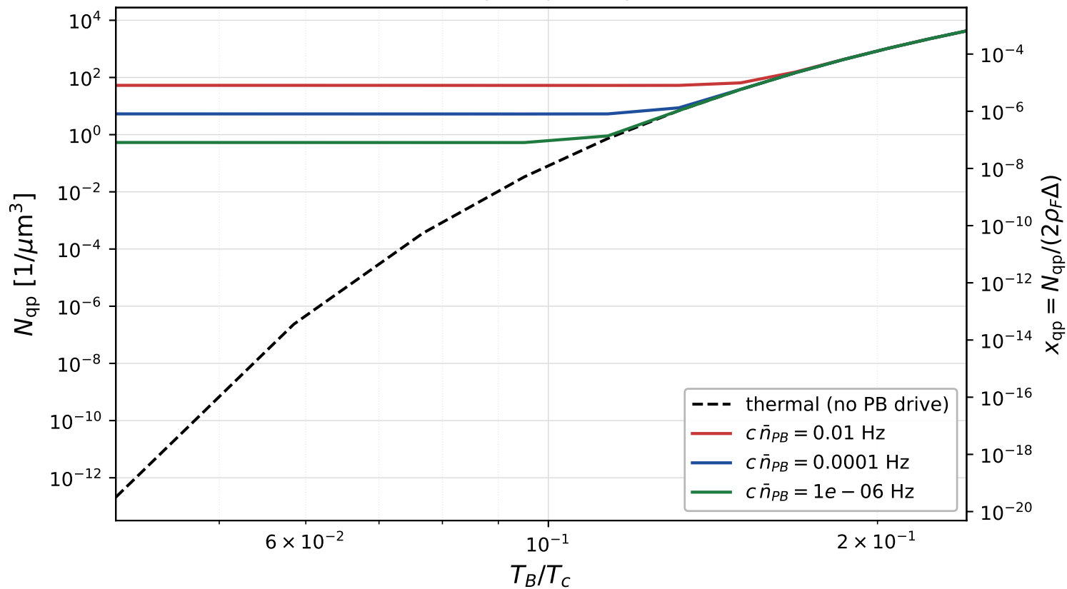
F24 Fig. 8 topology only — qpsim-native numerical curves Drive levels borrowed from the Fig. 5 caption; Fig. 8 inset values are unverified
