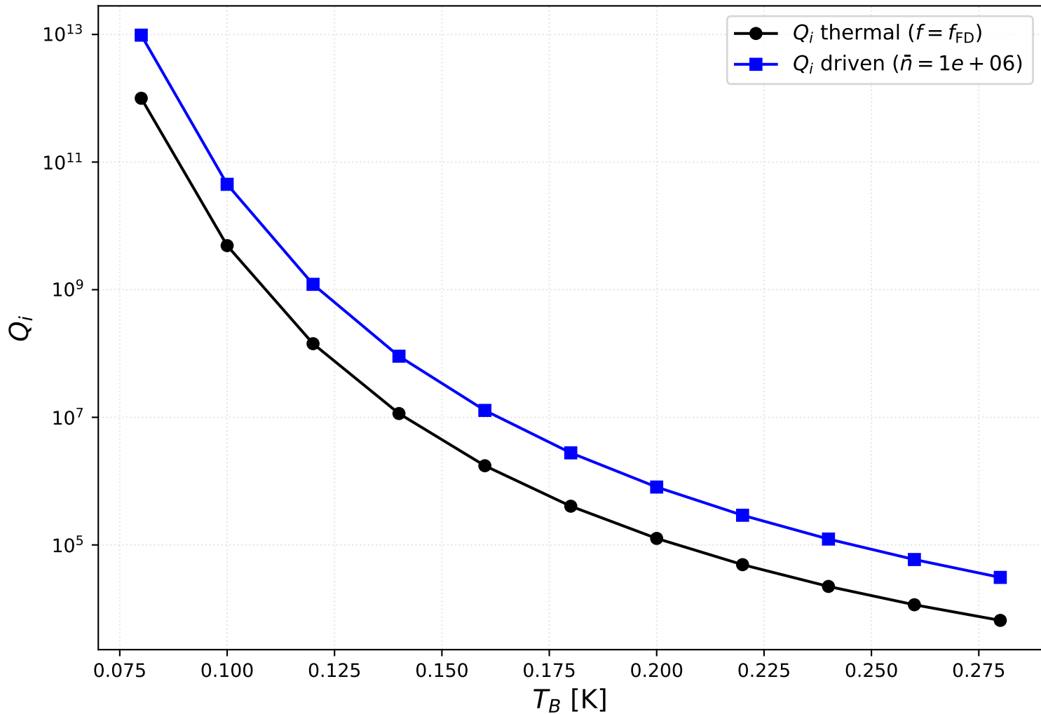
Fischer 2023 Fig 7 — Q_i(T_B) fixed- \bar{n} drive \Delta_0 = 180 \mu\text{eV} , \omega_0 = \Delta_0/9 , \alpha = 0.5 , c_{\text{phot}} = 1 \text{ Hz}
