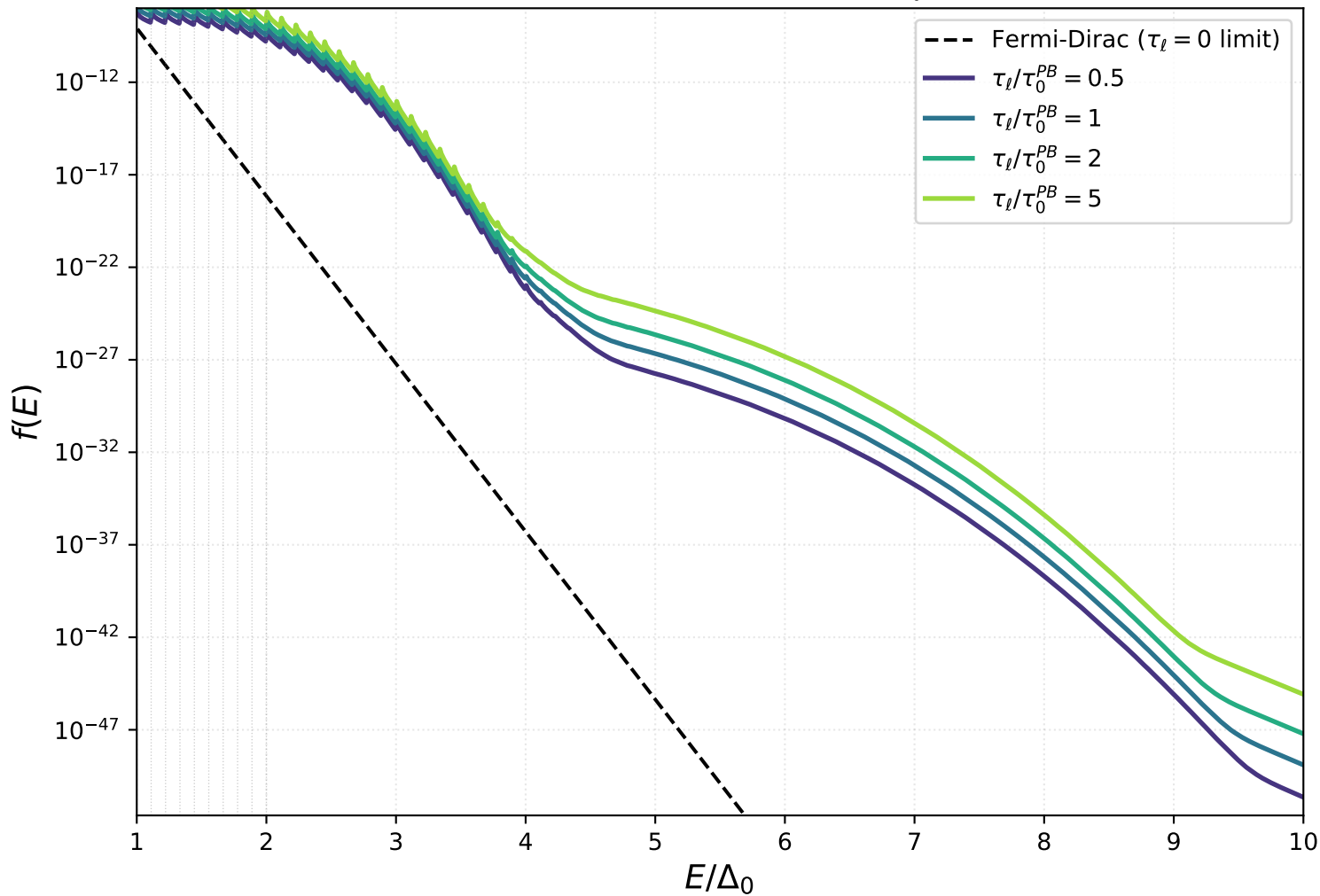
Fischer 2023 Fig 3 — finite- \tau_\ell (Ph0-constant) \Delta_0 = 180 \text{ } \mu\text{eV} , \omega_0 = \Delta_0/9 , \bar{n} = 10^7 , T_B = 0.1 \text{ K} , \tau_0^{PB} = 9.837 \text{ ns}
