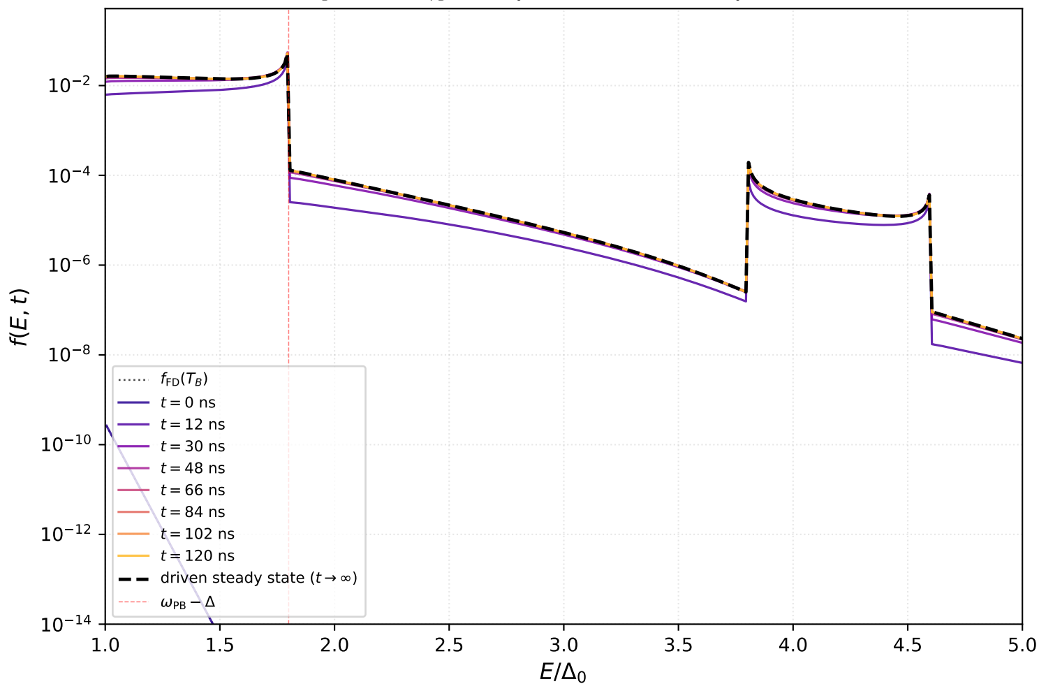
Photon-kick response: f(E, t) climbs toward the driven steady state
