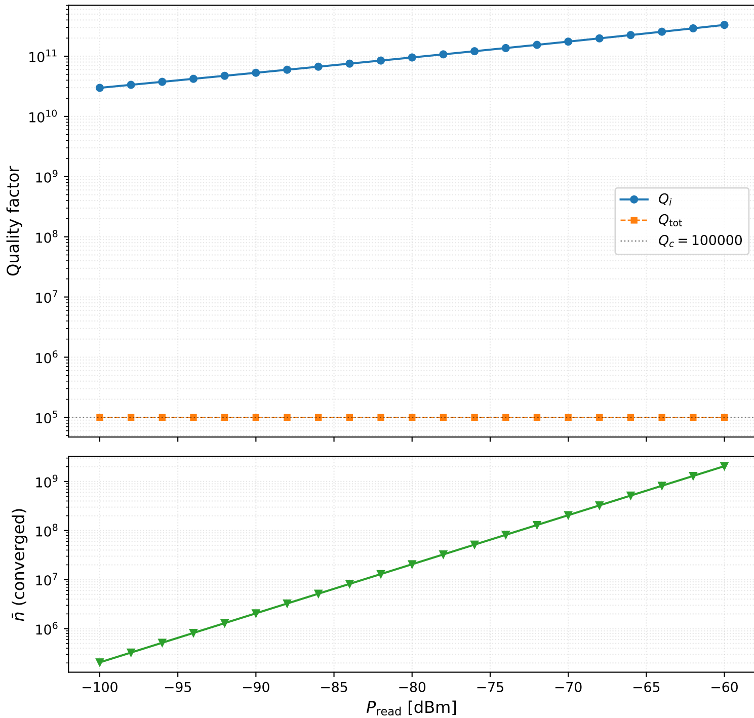
Fischer 2023 Figs 9-13 — Q_i(P_{\text{read}}) via \bar{n} loop \Delta_0 = 180 \text{ } \mu\text{eV} , \omega_0 = \Delta_0/9 , \alpha = 0.5 , Q_c = 100000 , T_B = 0.1 \text{ K}
