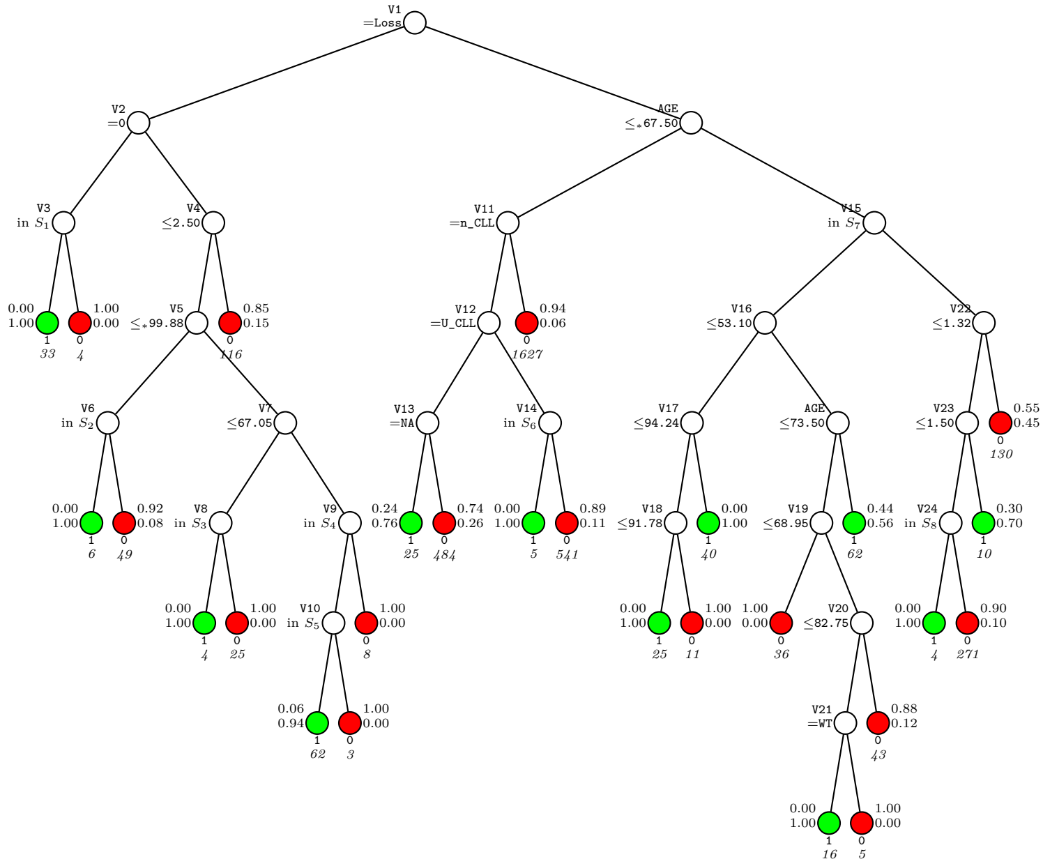
GUIDE v.46.2 0.250-SE classification tree for predicting death_5yr using estimated priors and unit misclassification costs. At each split, an observation goes to the left branch if and only if the condition is satisfied. Symbol ' \leq_{\cdot} ' stands for ' \leq or missing'. V1 = X17p_status. V2 = CLL_EPITYPE. V3 = tri12_status. V4 = RAI_AT_SAMPLING. V5 = IGHV_IDENTITY_PERCENTAGE. V6 = PRIOR_TREATMENT_CATEGORY. V7 = NORMAL_MEAN_COVERAGE. V8 = PRIOR_TREATMENT_CATEGORY. V9 = X18p_status. V10 = X8q_status. V11 = CLL_EPITYPE. V12 = TUMOR_MOLECULAR_SUBTYPE. V13 = U1_STATUS. V14 = PRIOR_TREATMENT_CATEGORY. V15 = EXPRESSION_CLUSTER. V16 = TUMOR_MEAN_COVERAGE. V17 = IGHV_IDENTITY_PERCENTAGE. V18 = IGHV_IDENTITY_PERCENTAGE. V19 = NORMAL_MEAN_COVERAGE. V20 = NORMAL_MEAN_COVERAGE. V21 = U1_STATUS. V22 = TMB_NONSYNONYMOUS. V23 = RAI_AT_DIAGNOSIS. V24 = PRIOR_TREATMENT_CATEGORY. S_1 = \{\text{Unchanged}\} . S_2 = \{\text{Chemo\_+\_no\_Ab}\} . S_3 = \{\text{Chemo\_+\_Ab}\} . S_4 = \{\text{Unchanged}\} . S_5 = \{\text{Unchanged}\} . S_6 = \{\text{Chemo\_+\_no\_Ab}\} . S_7 = \{\text{EC\_m1, EC\_m2, EC\_u1, EC\_u2}\} . S_8 = \{\text{Chemo\_+\_no\_Ab}\} . Predicted class and sample size (in italics ) printed below each terminal node; class posterior probabilities for death_5yr = 0 and 1 beside node. Second best split variable at root node is U.CLL_WES.
