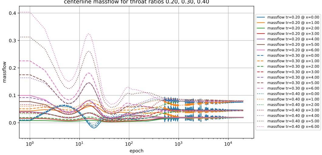
Figure 4: Mass flow at 7 centerline locations, obtained by integration over the corresponding cross-sectional area as described by Eqn. (22), for 3 different throat ratios \mathcal{G} (see Eqn. (15)), denoted in the legend as "tr".
