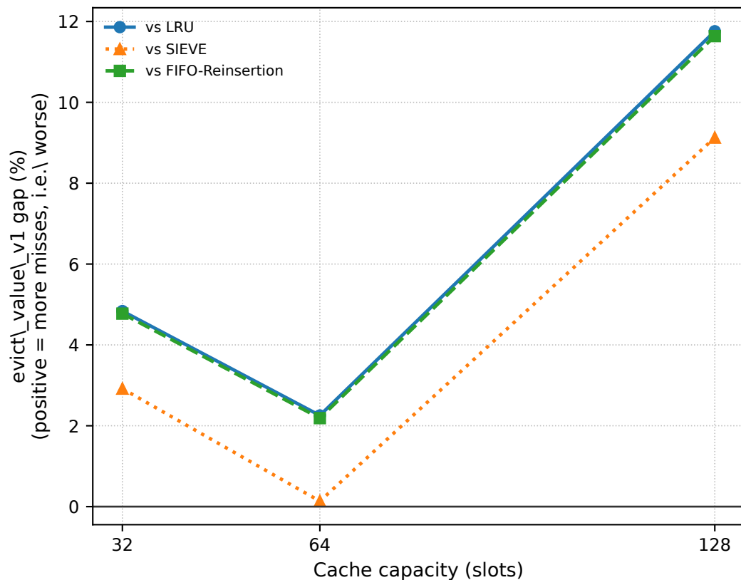
(b) evict_value_v1 gap vs baselines
