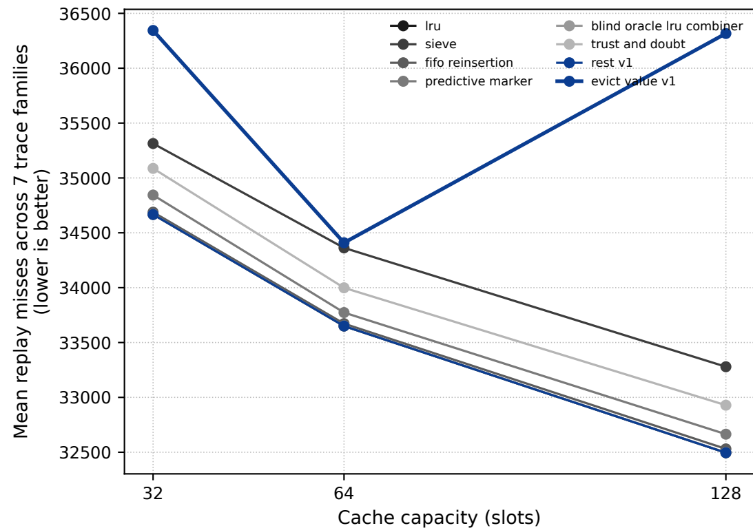
(a) Mean misses by capacity
