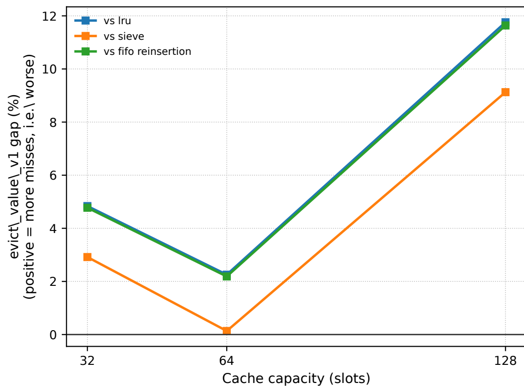
(b) evict_value_v1 gap vs baselines
