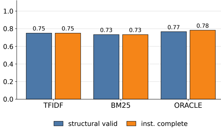
Fig. 2 Structural-validity and instantiation-completeness rates on the 60-instance engineering subset, for TF-IDF, BM25, and Oracle schema retrieval.
