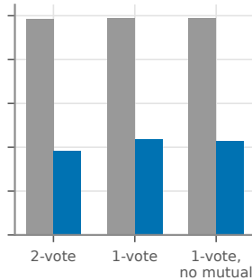
HotpotQA
