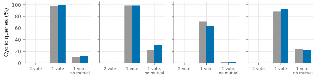
HotpotQA
