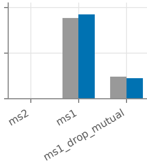
BRIGHT
