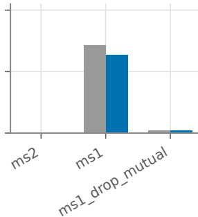
HotpotQA
