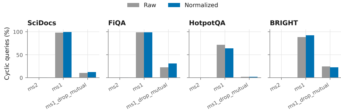
Fig. 4. Cyclic-query percentage by vote regime, raw-margin ablation (gray) versus primary normalized protocol (blue), one panel per dataset. Unlike the BM25 weight share in Figure 2, overall cyclic-query rate changes only modestly between raw and normalized construction within each regime. The reader should not conclude that normalization leaves the graph unchanged: Section 5 shows the removed-edge overlap between raw and normalized repair is only 0.055–0.328, so normalization changes which edges are cyclic and removed far more than it changes the headline cyclic-query rate shown here.
