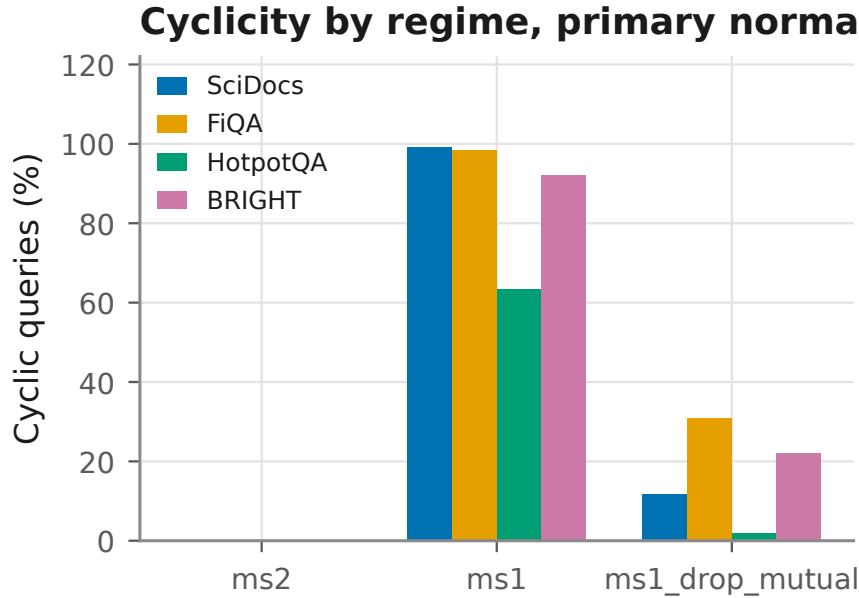
Fig. 3. Cyclic-query percentage under the primary normalized protocol, grouped by vote regime with one bar per dataset. ms2 is exactly 0% on every dataset; ms1 is 64–99%; deleting direct mutual pairs (ms1_drop_mutual) brings every dataset back down to 2–31%. The reader should notice that ms1’s high cyclicicity is concentrated almost entirely in direct mutual contradictions, not longer cycles – Figure 5 isolates that residual directly. Values before mutual-pair deletion; post-deletion values are also in Table 5.
