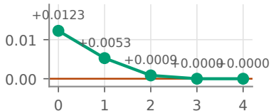
(A) HotpotQA
