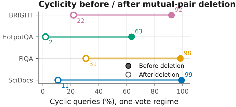
Fig. 2 Cyclic-query percentage under ms1 before and after deleting direct mutual pairs, by dataset. Most active-regime cyclicality is direct two-way contradiction, not longer-cycle structure, but a nonzero, dataset-dependent residual remains after mutual-pair deletion.
