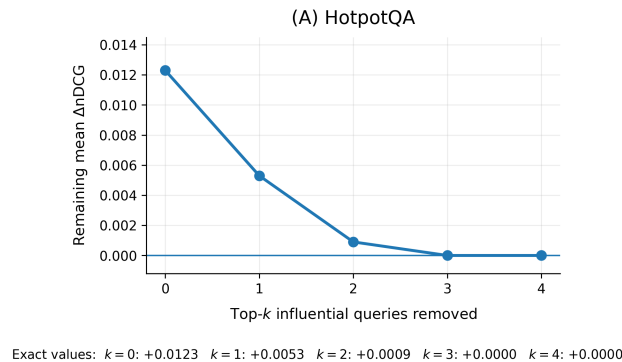
Fig. 8. Remaining mean \Delta nDCG for the calibrated ms1 Copeland-hybrid cell as the top- k most influential HotpotQA queries are removed ( k = 0, \dots, 4 ), the more concentrated of the two main positive-point-estimate cases. The mean falls from +0.0123 to exactly 0 after removing the top 3 queries, so the positive estimate is concentrated in a handful of queries. The companion SciDocs cell is less concentrated and is reported numerically in the text below rather than plotted here. Values are exact per-query recomputations, not interpolated.
