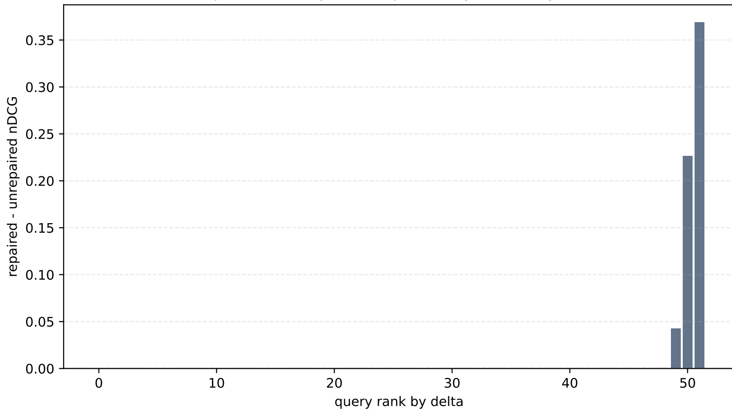
HotpotQA Primary ms1 Copeland-Hybrid Query Deltas
