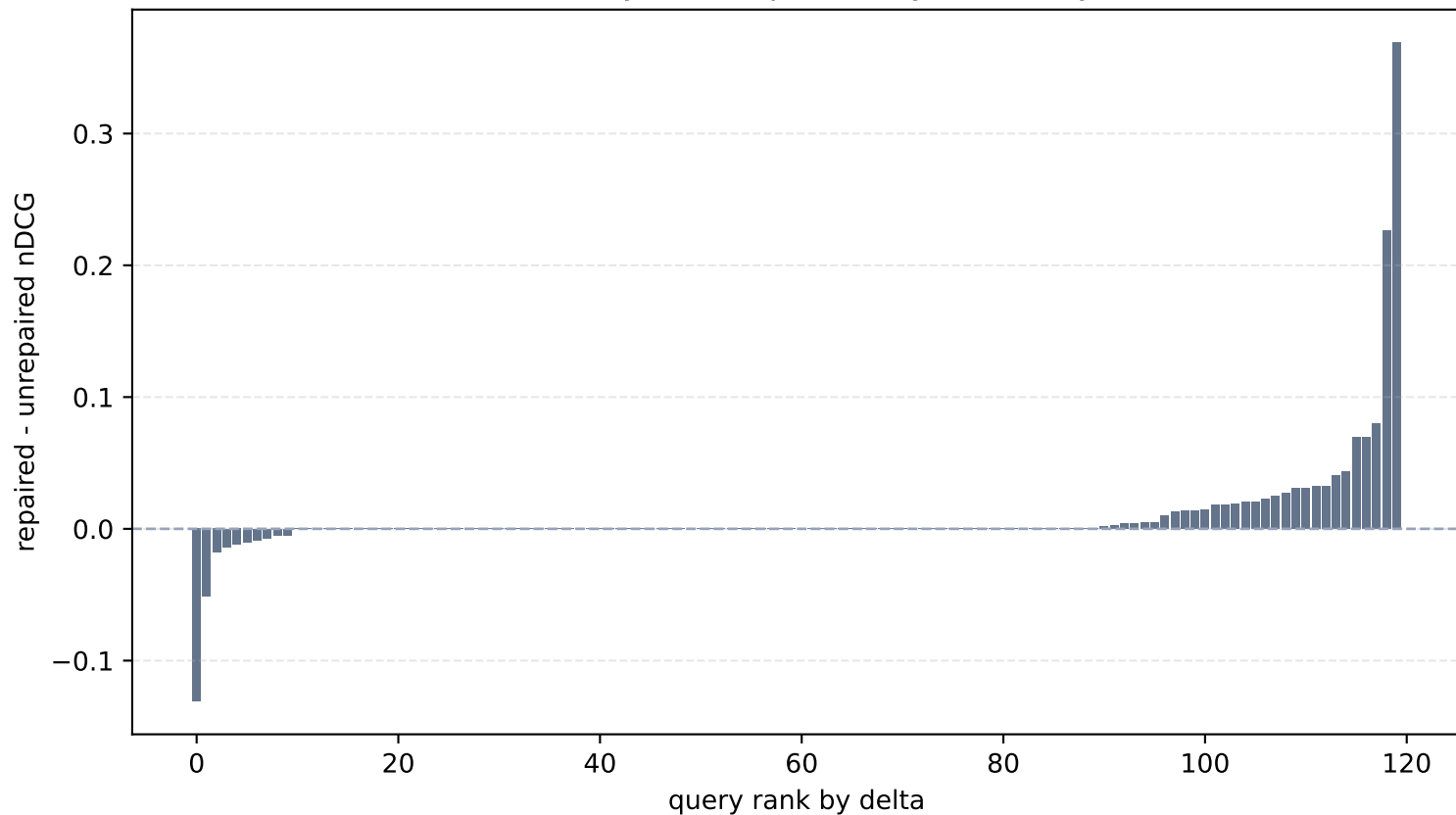
SciDocs Primary ms1 Copeland-Hybrid Query Deltas
