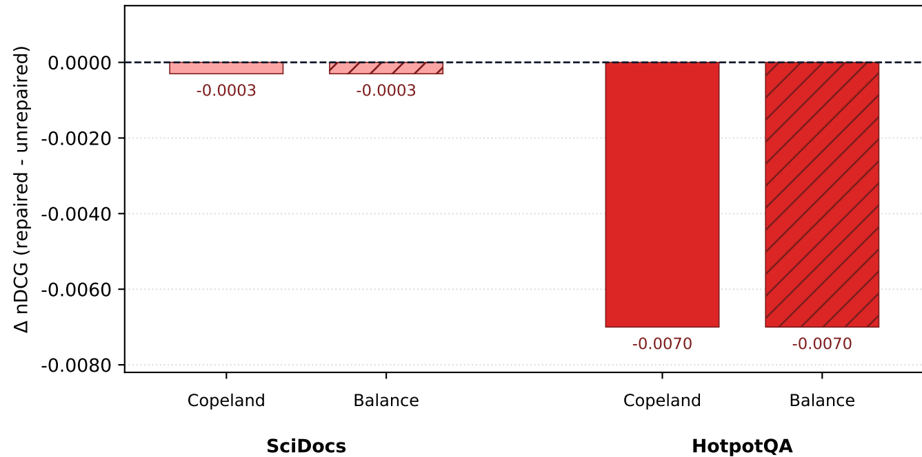
Repair effect on nDCG from tracked real pairwise runs
