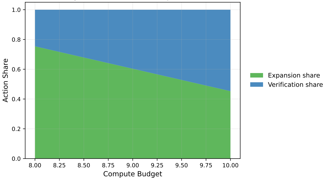
Figure 4: Allocation Composition
