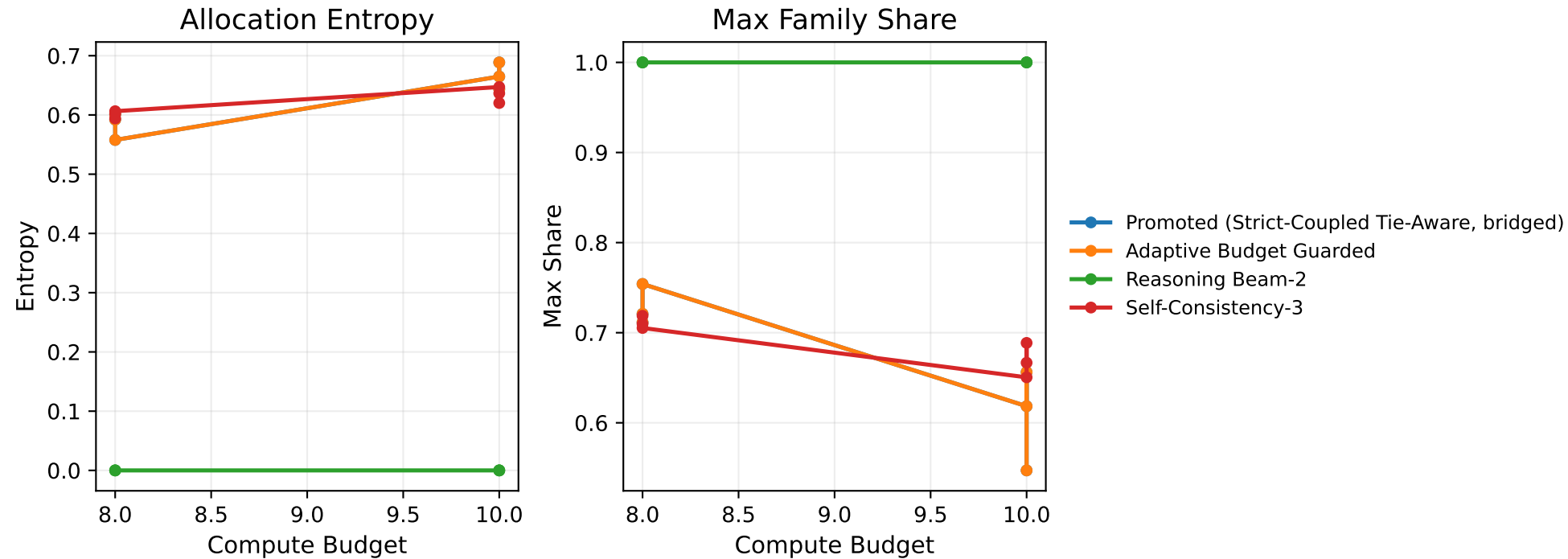
Figure 5: Anti-Collapse Diagnostics
