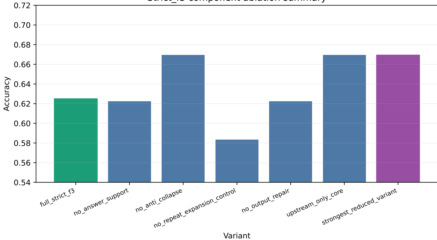
Strict_f3 component ablation summary
