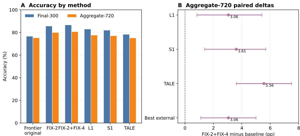
Figure 2: Main accuracy summary for the promoted policy. Panel A compares FIX-2+FIX-4 with the frontier baseline and external baselines on Final-300 and Aggregate-720. Panel B shows Aggregate-720 paired deltas for FIX-2+FIX-4 versus L1, S1, TALE, and the best external baseline; the zero line marks no improvement. The primary promoted evidence is the disjoint Final-300 and Aggregate-720 evaluation, and the figure is descriptive rather than a new claim.
