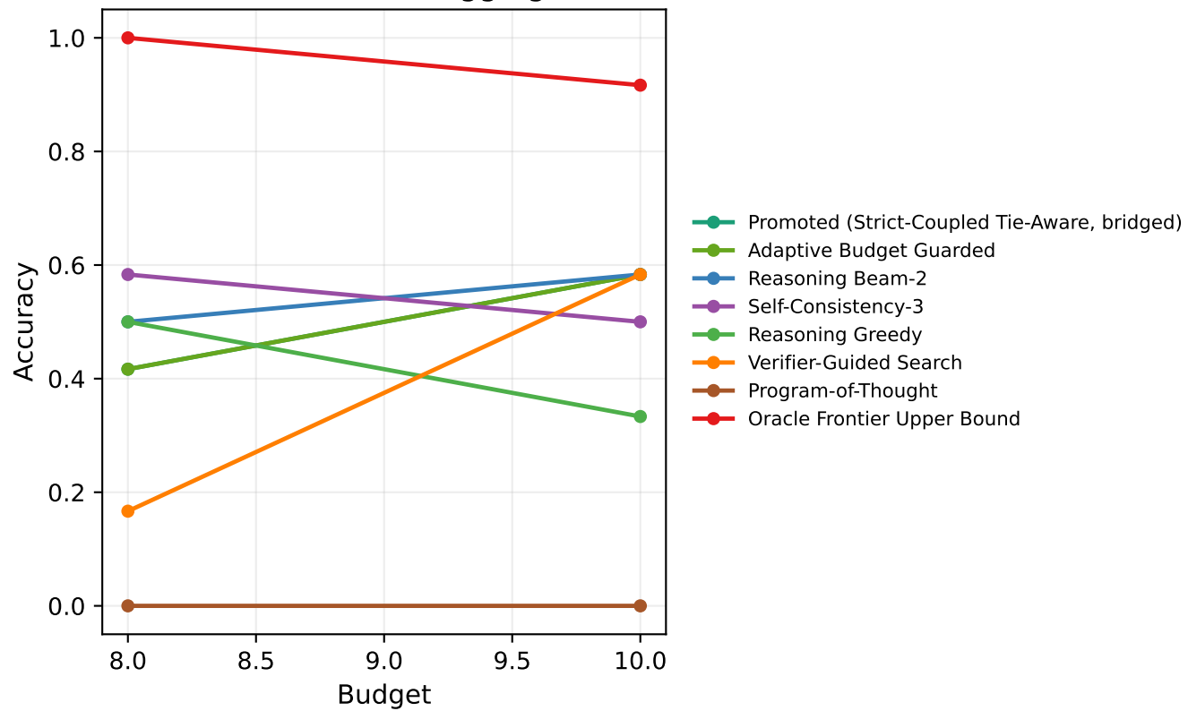
Appendix: Full Frontier Curves (HuggingFaceH4/MATH-500)
