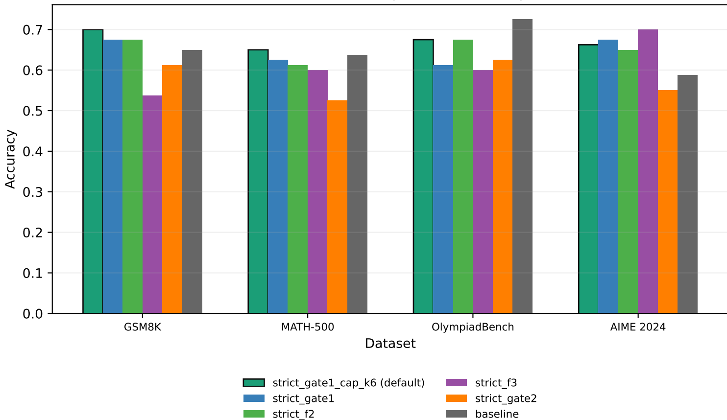
Per-dataset strict-phased summary
