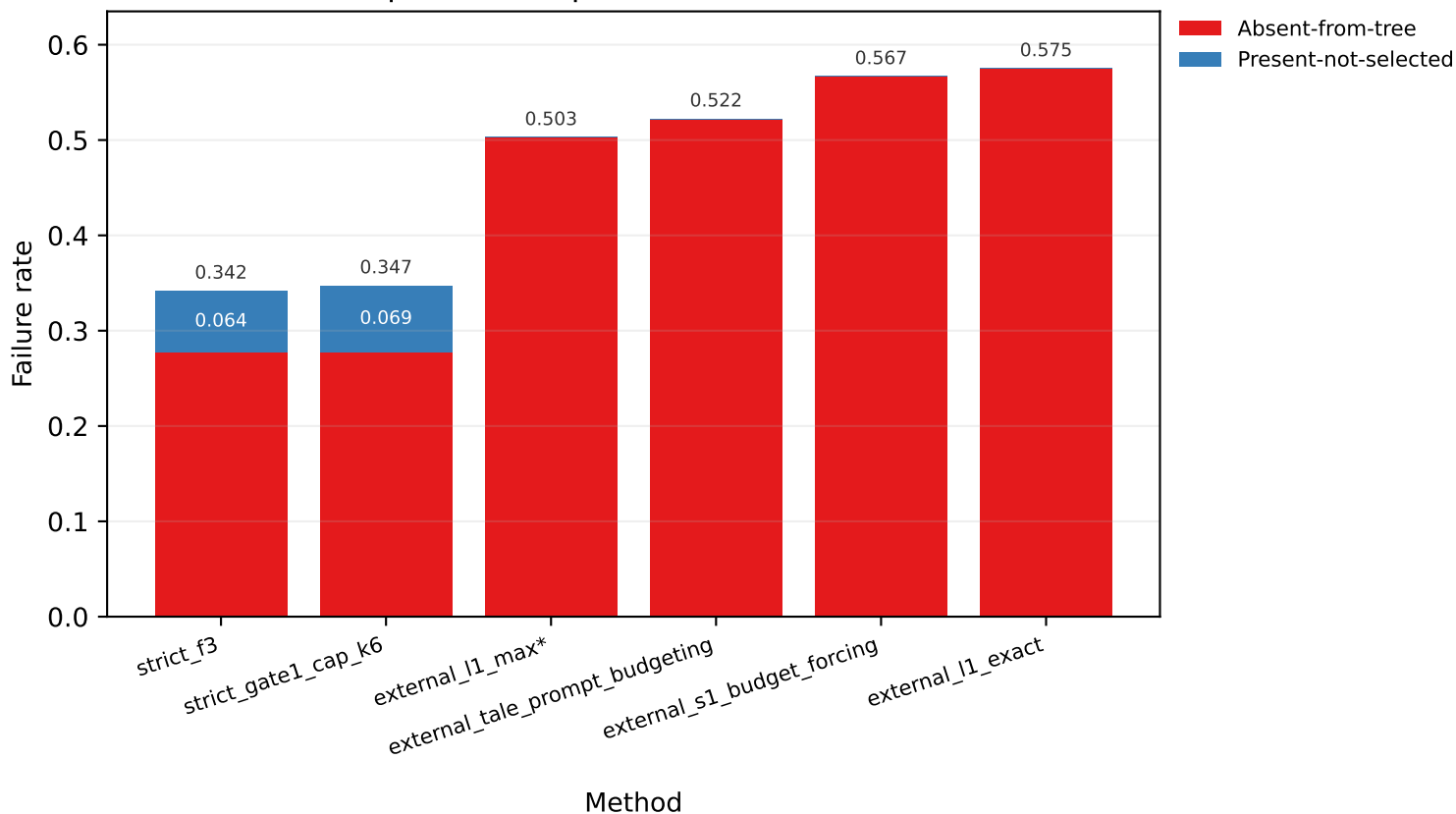
Failure decomposition (expanded fair near-direct externals)
