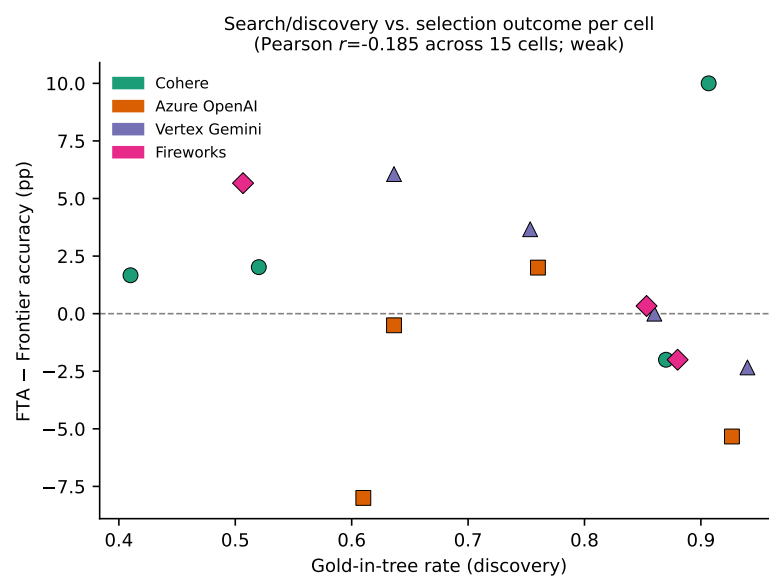
Figure O.5: Discovery rate vs. FTA–Frontier delta (15 cells). Global Pearson r = -0.185 (not supported at n=15 ); leave-one-out ranges vary. Descriptive sanity check; Azure sign reversal is the clearer tested instance (Section 8).
