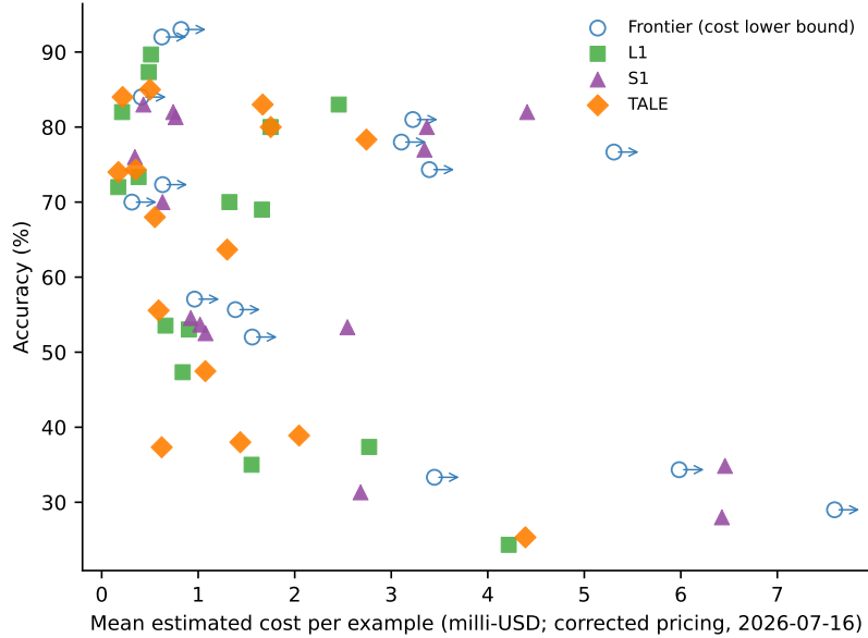
Figure 4: Class A accuracy vs. mean estimated cost per example (milli-USD) for the evaluated adapters under this protocol. Points occupy a tradeoff region. Open Frontier markers with rightward arrows mark incomplete challenger-phase token persistence.
