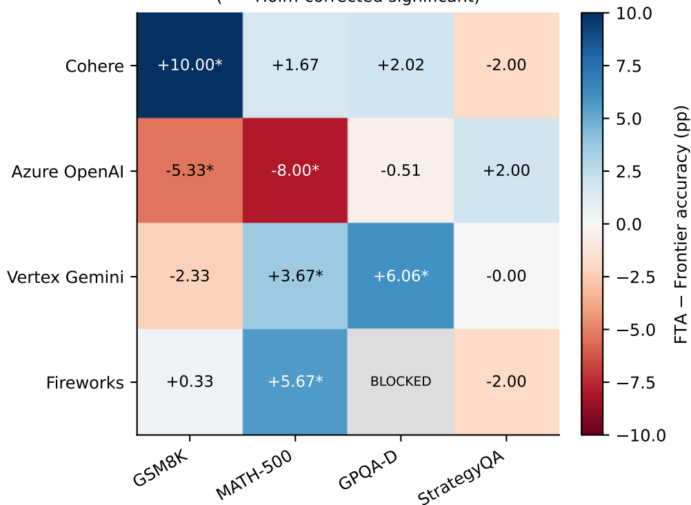
FTA vs. Frontier delta by provider × dataset (* = Holm-corrected significant)
