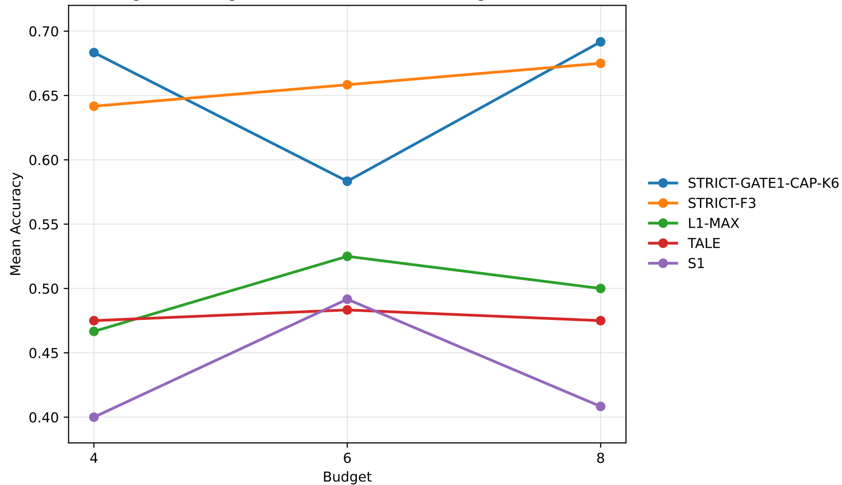
Figure 2: Budget-Performance Frontier (Budgets 4, 6, 8)
