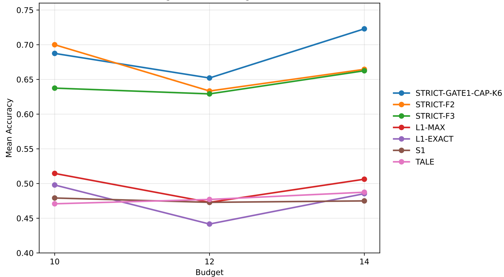
Extended-Budget Frontier (Budgets 10, 12, 14)
