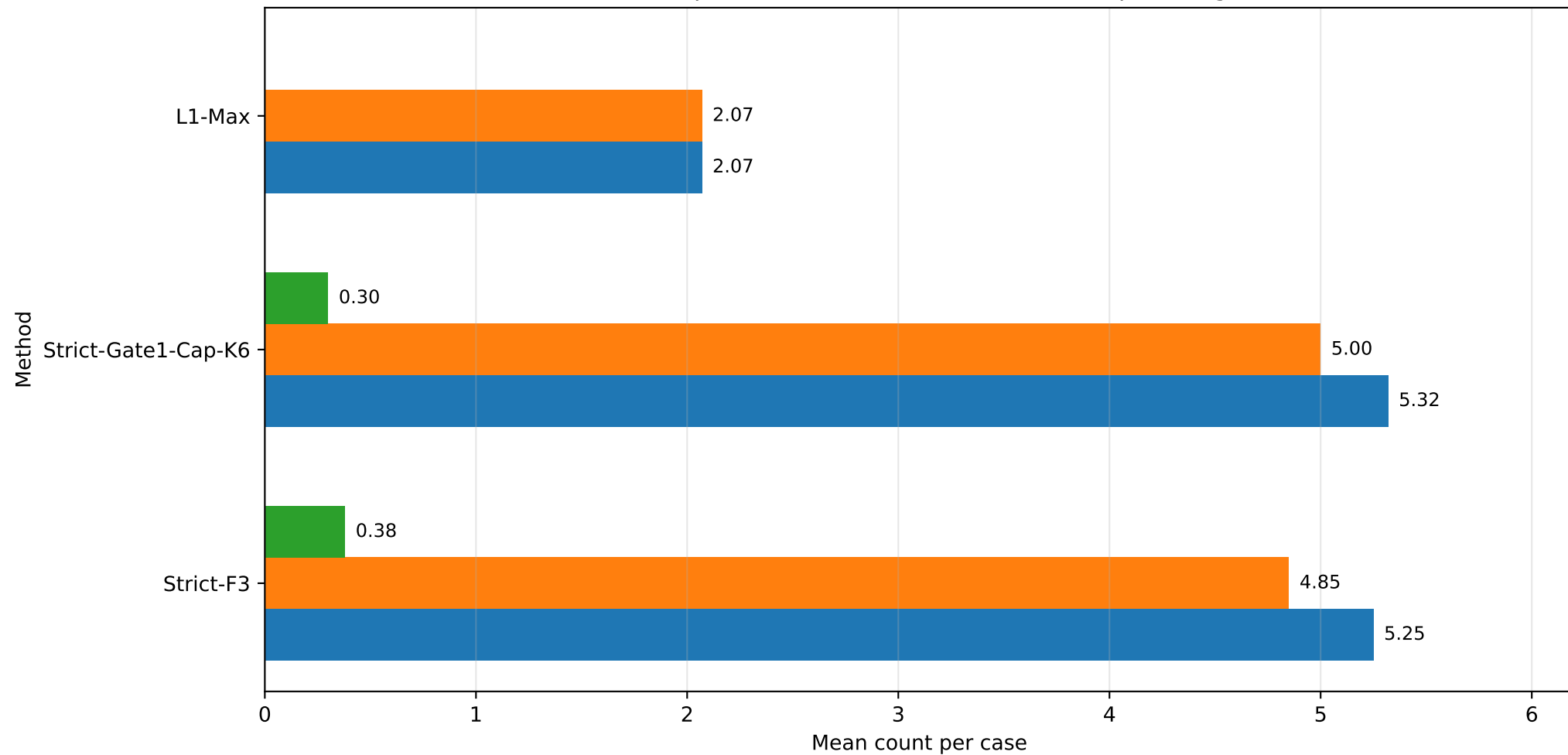
Avg actions Avg expansions Avg verifications Allocation composition on the matched manuscript-facing surface
