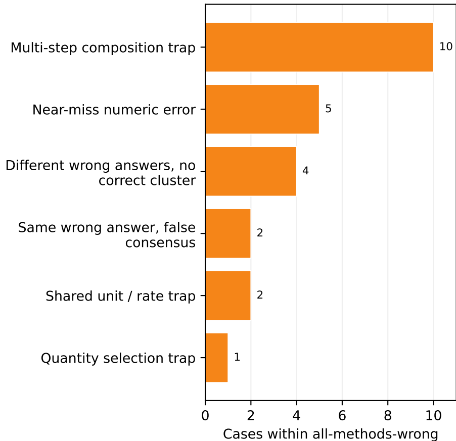
B All-methods-wrong subtypes
