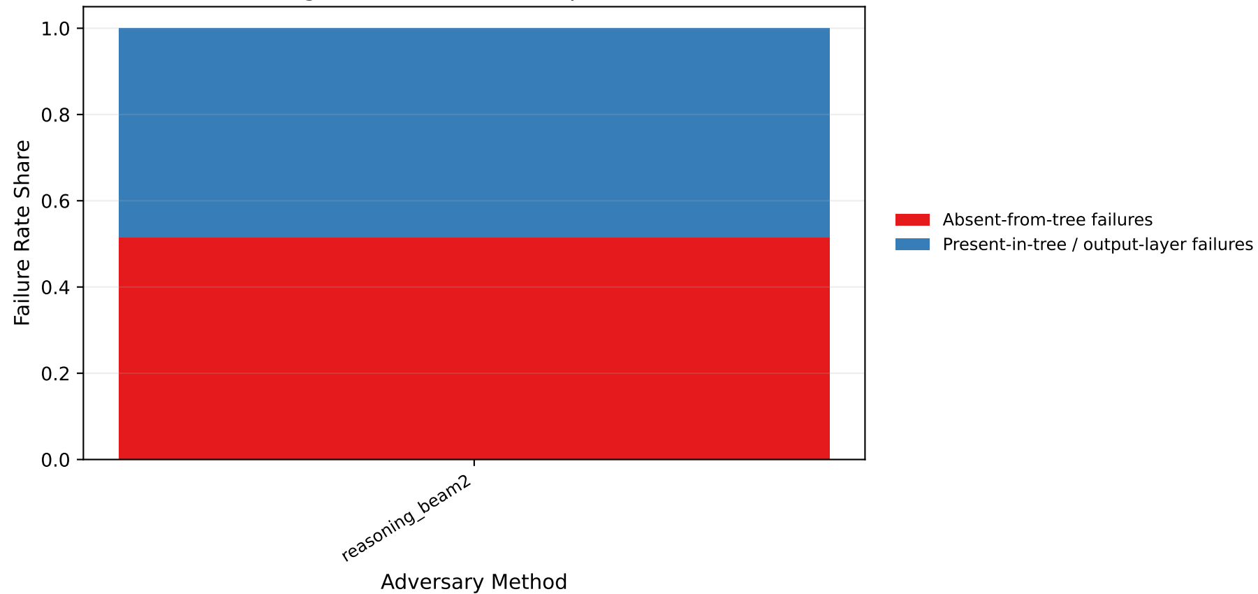
Figure 6: Failure Decomposition
