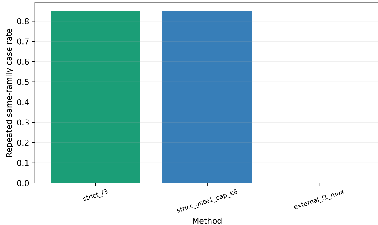
Anti-collapse diagnostic: repeated same-family case rate
