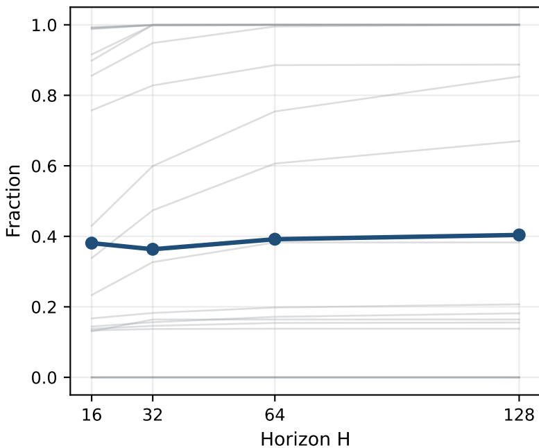
Discriminative fraction
