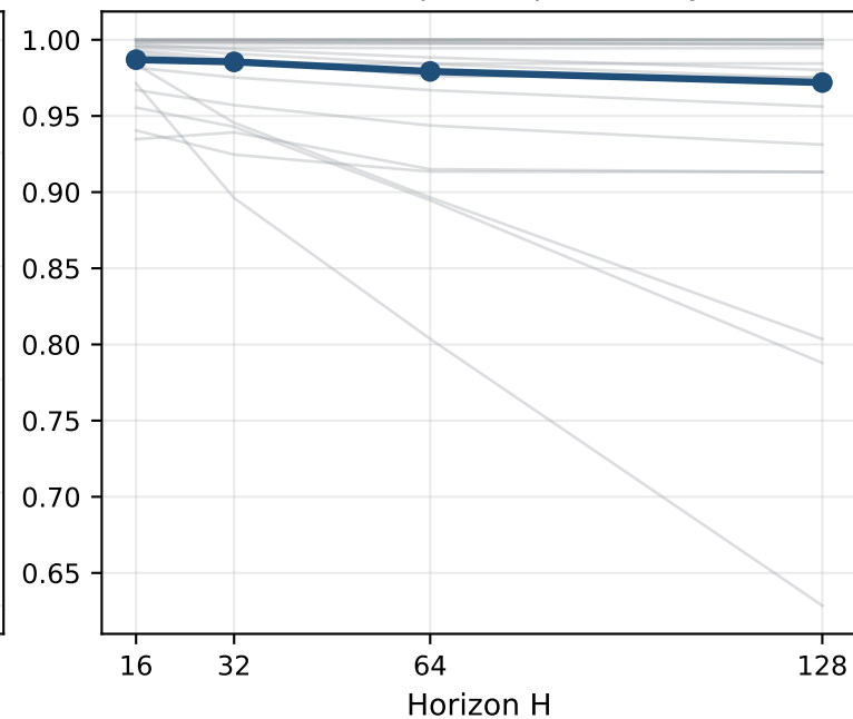
Random-optimal probability
