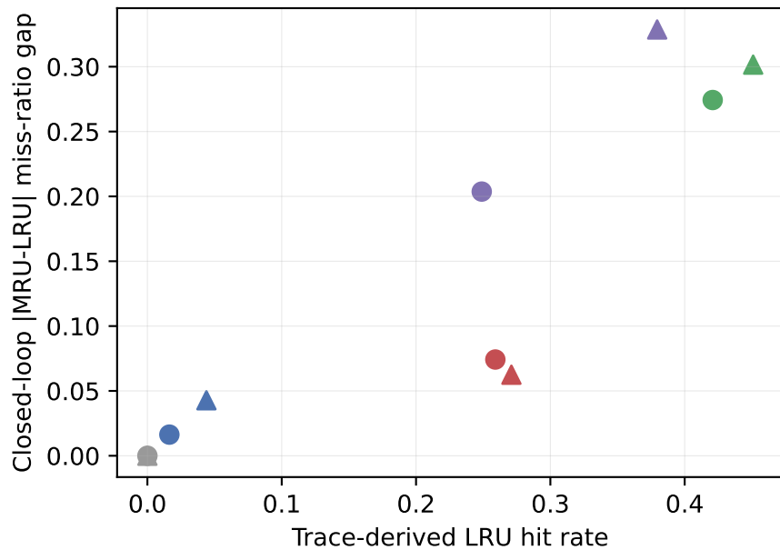
Locality vs. policy separation ( r=0.90 , n=10 )
