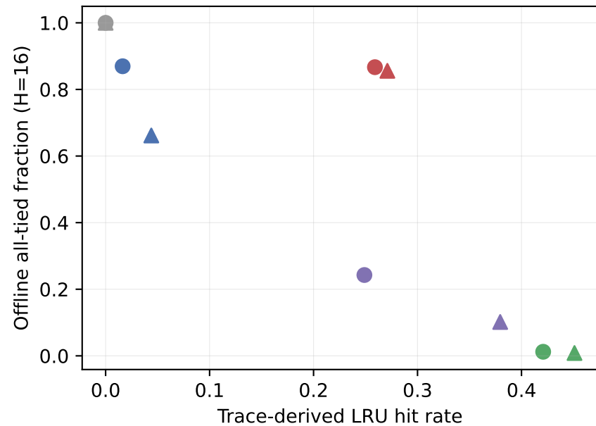
Locality vs. tie rate ( r=-0.83 , n=10 )
