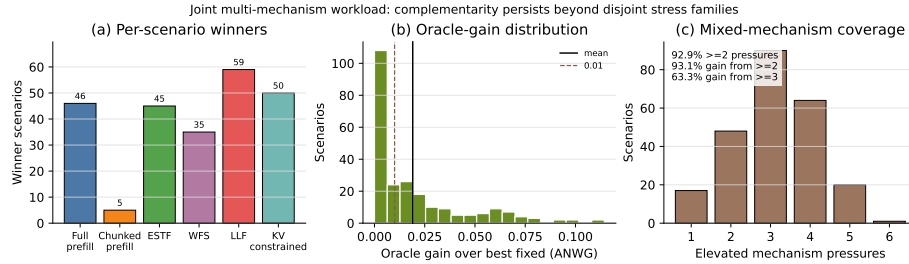
Fig. 1. Joint multi-mechanism workload results. The portfolio retains winner diversity, positive oracle gain, and gain concentrated in scenarios with multiple elevated mechanism pressures.
