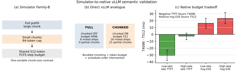
Fig. 2. Real-vLLM semantic validation. A direct Family-B mapping bundles chunking and scheduler-token-budget changes, while the native vLLM budget probe keeps chunked prefill enabled and varies only max_num_batched_tokens . Differences are T4096 minus T512; negative late TTFT favors T4096, positive hog E2E favors T512.
