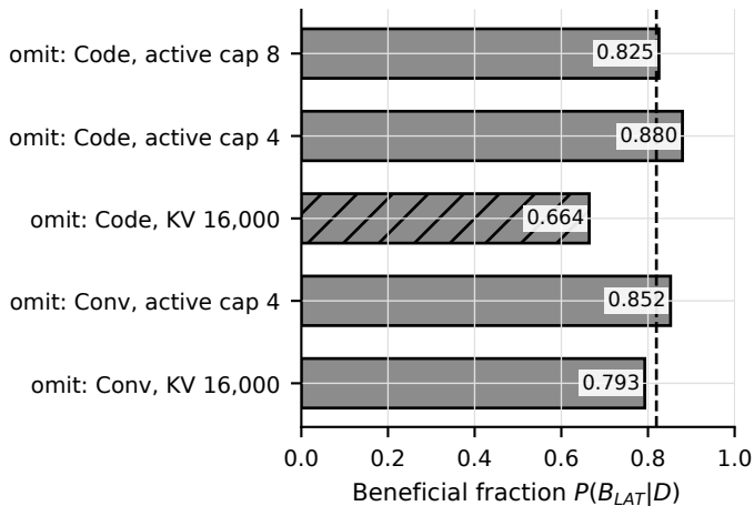
(c) Leave-one-regime-out: beneficial fraction
