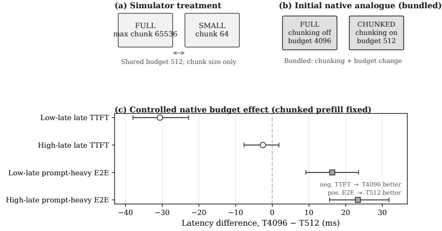
Fig. 2. Simulator-to-native vLLM validation on the local probe. (a) Simulator Family-B-style treatment: shared 512-token step budget; only prefill chunk size varies (FULL vs. SMALL). (b) Initial native analogue: chunking and token budget change together (bundled; not a single-factor contrast). (c) Controlled native experiment with chunked prefill fixed; plotted points are T4096–T512 latency differences with 95% bootstrap CIs. Negative late-request TTFT favors T4096; positive prompt-heavy E2E favors T512.
