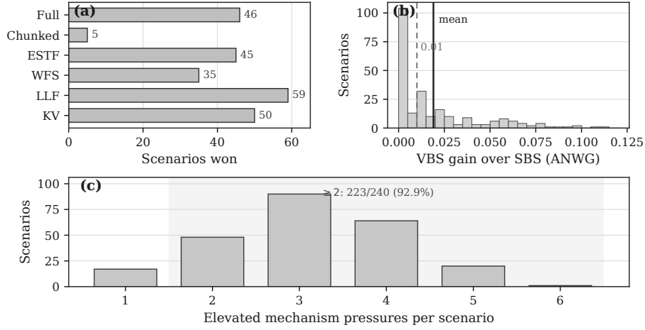
Fig. 1. Joint 240-scenario multi-mechanism workload under the canonical six-policy portfolio P_6 (this figure does not include the external expansion in Section 3.4). (a) Per-scenario VBS winner counts (Full, Chunked, ESTF, WFS, LLF, KV). (b) Distribution of per-scenario VBS gain over the SBS (ANWG); solid line is mean headroom, dashed line is 0.01. (c) Elevated mechanism pressures per scenario (threshold 0.60); shaded region marks \geq 2 pressures. Winner diversity and positive VBS headroom persist under jointly varying pressures.
