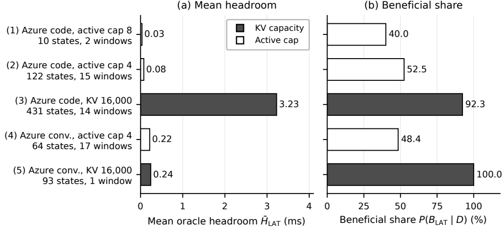
Figure 4: Fresh causal characterization of the five selected regimes, numbered as in Table 3 (conv. = conversation; active cap = active-sequence cap; KV = KV capacity in tokens). (a) State-weighted mean oracle headroom \bar{H}_{LAT} within each regime (ms). (b) Beneficial share P(B_{LAT} | D) : the percentage of the regime’s disagreement states with positive headroom under the preregistered criterion. Fill denotes the pressure axis. State and window counts are shown in place of intervals, because window-clustered intervals are undefined for regimes with one or two windows.
