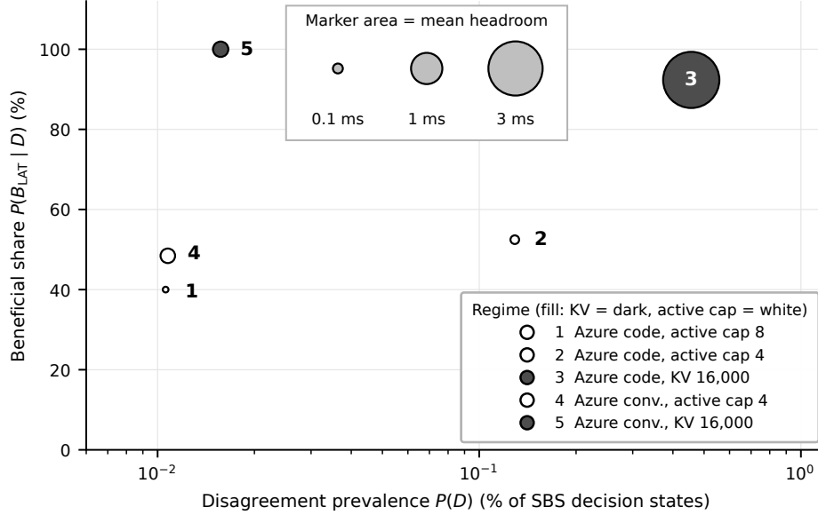
Figure 5: Regime map for the five selected regimes, numbered as in Figure 4 and Table 3. Horizontal axis: disagreement prevalence P(D) , the percentage of SBS decision states that are disagreement states (logarithmic scale). Vertical axis: beneficial share P(B_{LAT} | D) . Marker area is proportional to the regime’s mean oracle headroom (key in the plot), and fill denotes the pressure axis. P(B_{LAT} | D) counts any positive headroom: regime 5, at 100%, has a mean headroom of 0.24 ms and a maximum below 0.48 ms.
