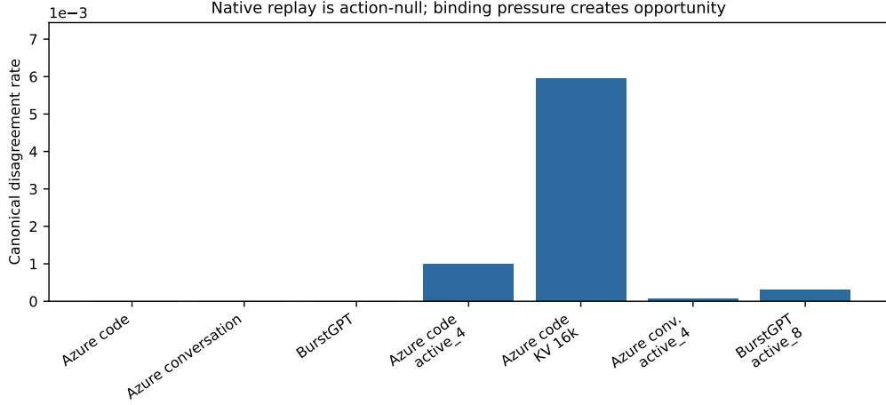
Figure 2: Canonical disagreement rate P(D) (fraction of SBS decision states) for native replay of the three workloads and for selected pressure conditions: Azure code with active-sequence cap 4 and with KV capacity 16,000 tokens (16k), Azure conversation with cap 4, and BurstGPT with cap 8.
