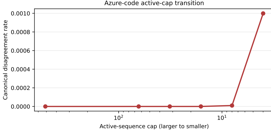
Figure 3: Canonical disagreement rate P(D) (fraction of SBS decision states) for Azure code as the active-sequence cap is tightened; the horizontal axis is logarithmic and reversed, so tighter caps lie to the right.
