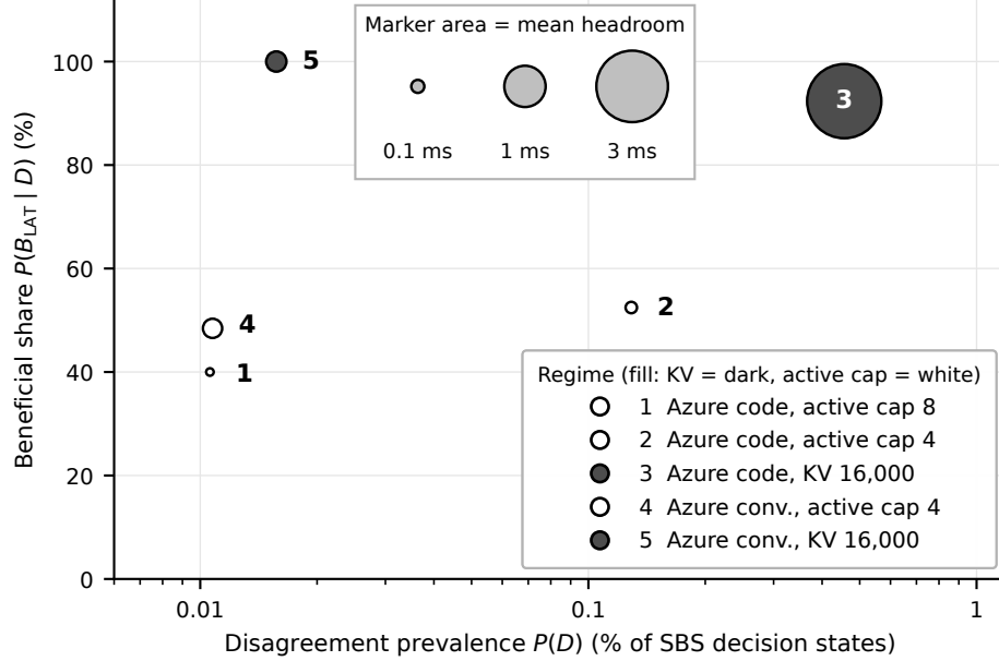
Figure 3: Regime map for the five selected regimes, numbered as in Table 3. Horizontal axis: disagreement prevalence P(D) in percent (logarithmic scale). Vertical axis: beneficial share P(B_{LAT} | D) , which counts any positive headroom (regime 5, at 100%, has a mean headroom of 0.24 ms). Marker area is proportional to the mean oracle headroom; fill denotes the pressure axis.
