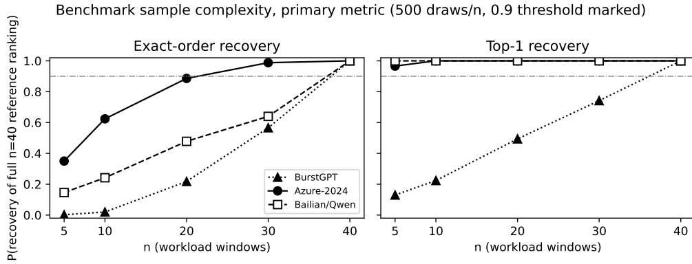
Figure 3: Benchmark sample-complexity recovery curves, PRIMARY metric, 500 draws per n , sampling without replacement. Left: exact-order recovery of the full n = 40 reference ranking. Right: top-1 recovery. The 0.9 threshold is marked. Computed from the frozen sample complexity artifact.
