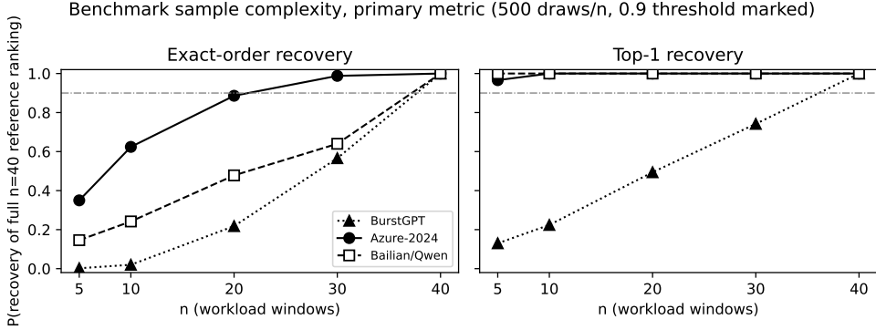
Fig. 3 Benchmark sample-complexity recovery curves, PRIMARY metric, 500 draws per n , sampling without replacement. Left: exact-order recovery of the full n = 40 reference ranking. Right: top-1 recovery. The 0.9 threshold is marked. Computed from the frozen sample complexity artifact.
