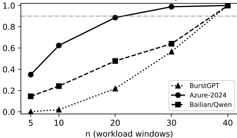
Exact-order recovery
