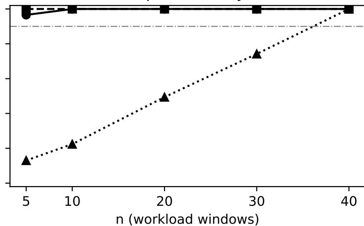
Top-1 recovery
