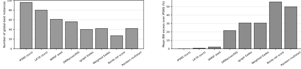
Fig. 2: Primary sparse-benchmark comparison. Left: best-count summary with ties credited to every tied method. Right: relative backward-weight behavior on the sparse comparison set. The figure visualizes the same accounting rules reported in Table 5.
