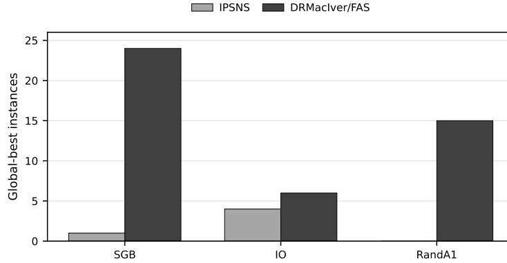
Fig. 3: Dense LOLIB transfer study. The selected complete-ordering benchmark favors the evaluated matrix-based DRMacIver/FAS implementation, marking a scope boundary for the sparse-digraph refinement strategy studied in this paper.
