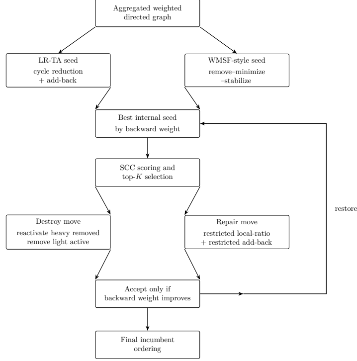
Fig. 1: Overview of the incumbent-protected SCC-neighborhood search framework. The method starts from the better of two attributed constructive seeds, scores cyclic strongly connected components by their current backward-weight contribution, applies component-local destroy-and-repair, and accepts only strict global improvements.
