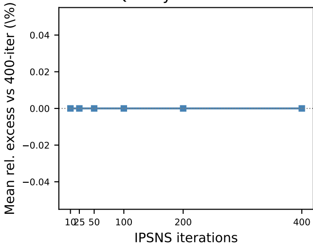
Quality saturation
