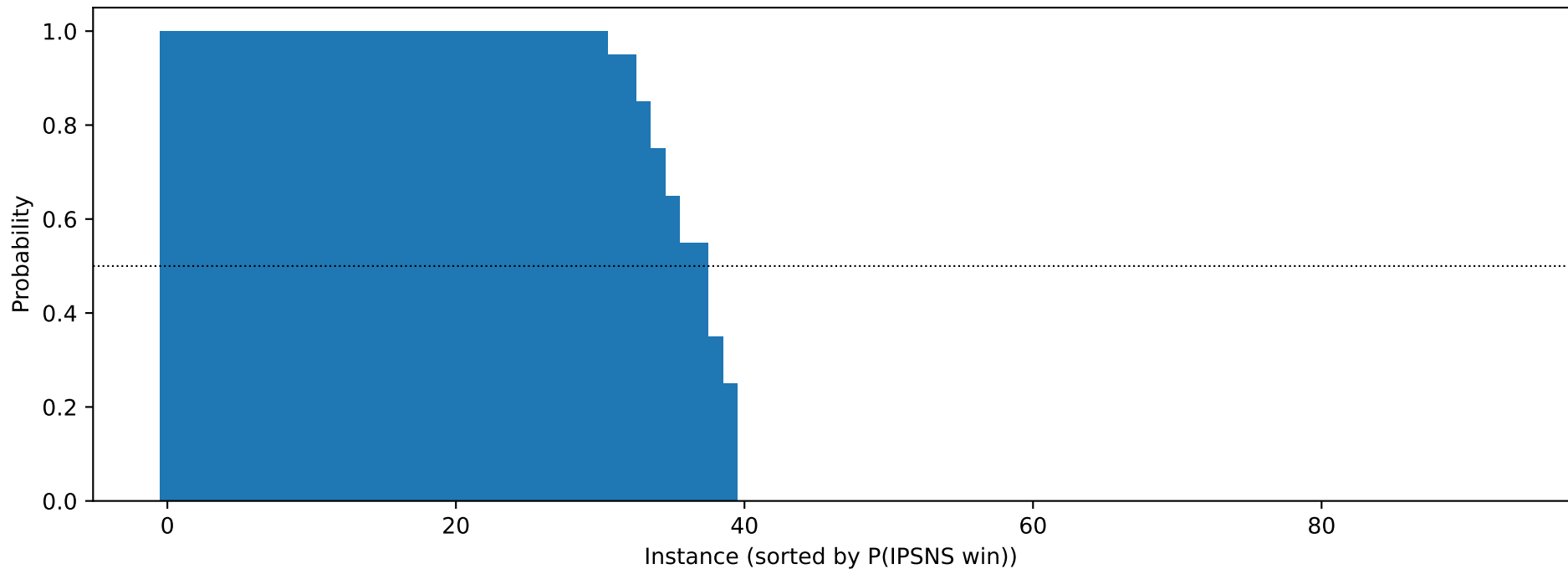
Per-instance P(\text{IPSNS} < \text{DR}) across cross-pairs
