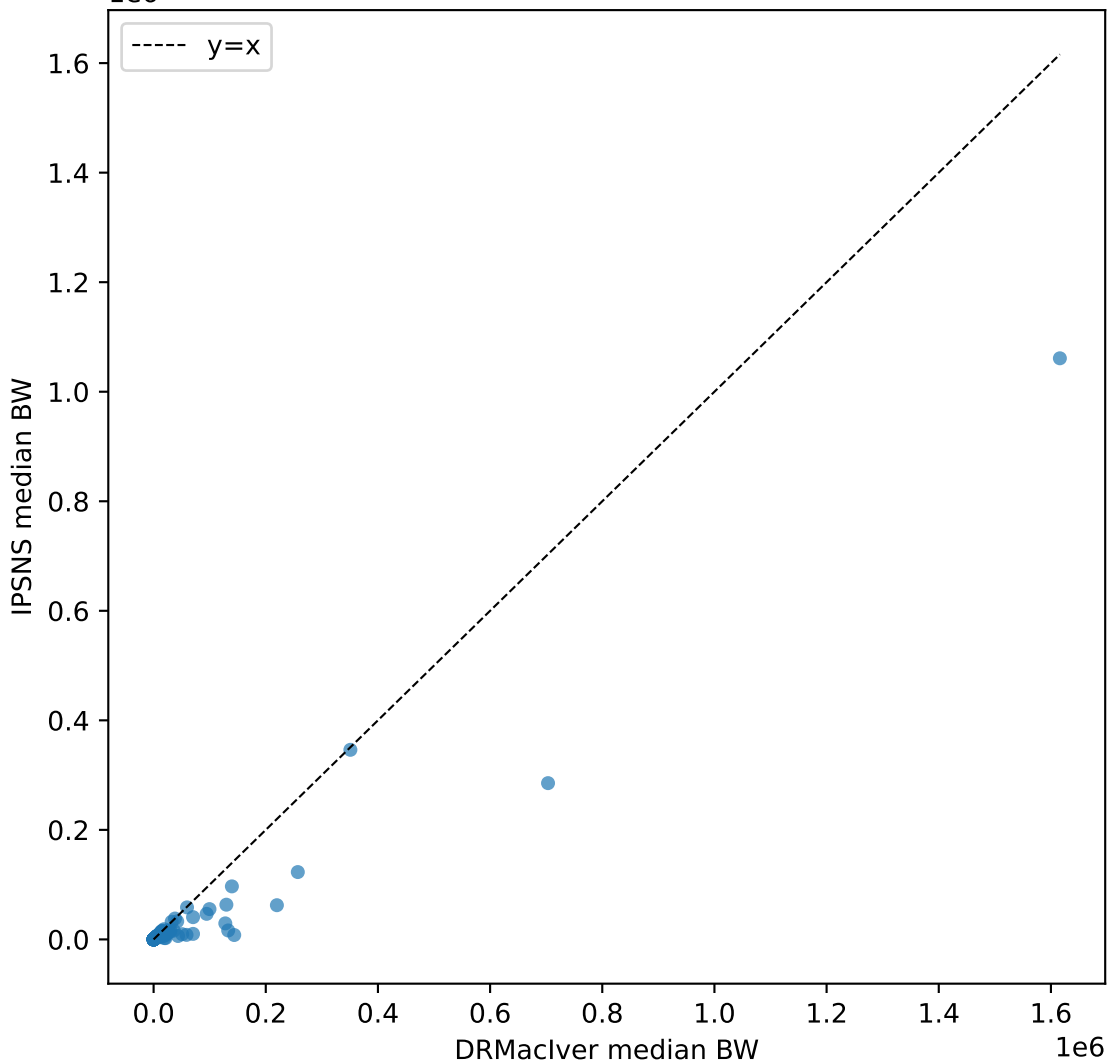
Per-instance medians (93 common instances)
